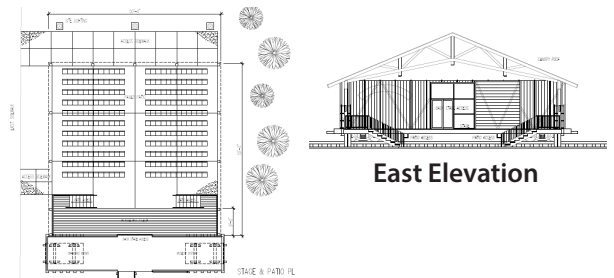
Stage & Patio Plan
